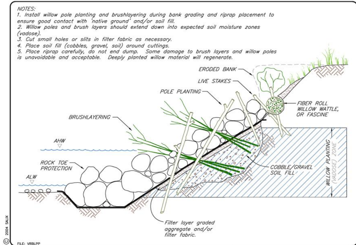
Figure 28. Vegetated riprap with brush layering and pole planting (Reprinted with permission from McCullah & Gray 2005).
